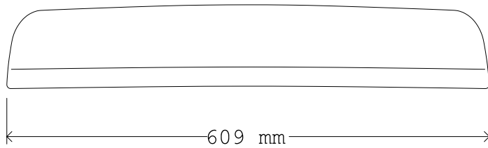
Streamline 24 magnetic roof sign illuminated
